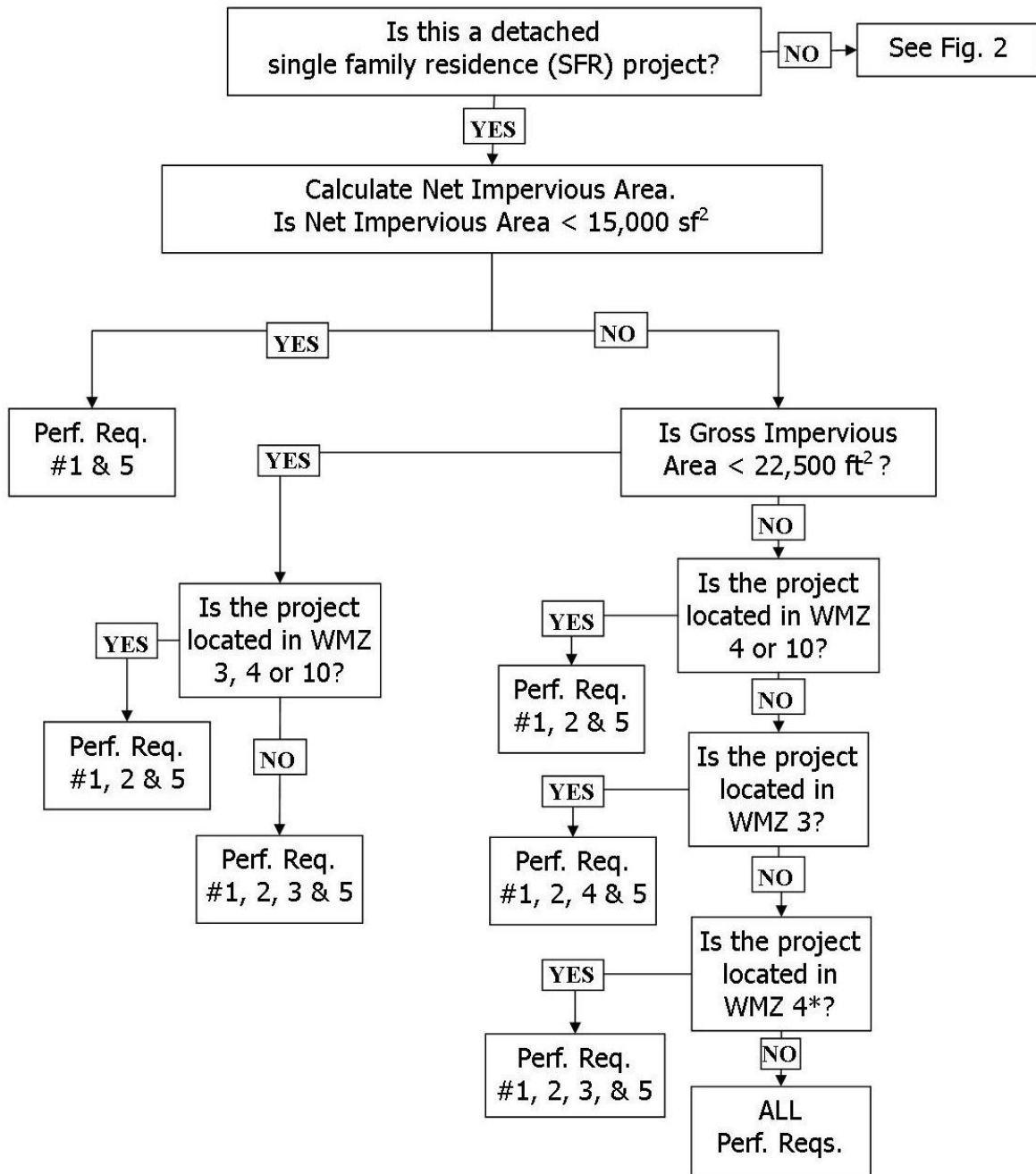
Performance Requirements Flow Chart for non-exempt projects
